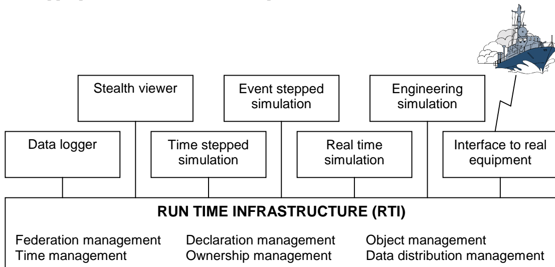
Figure 3: A functional view of the HLA. Many different types of federates may operate together over a network. The RTI provides the services that facilitate transfer of data amongst federates and the co-ordination of their time advances.
