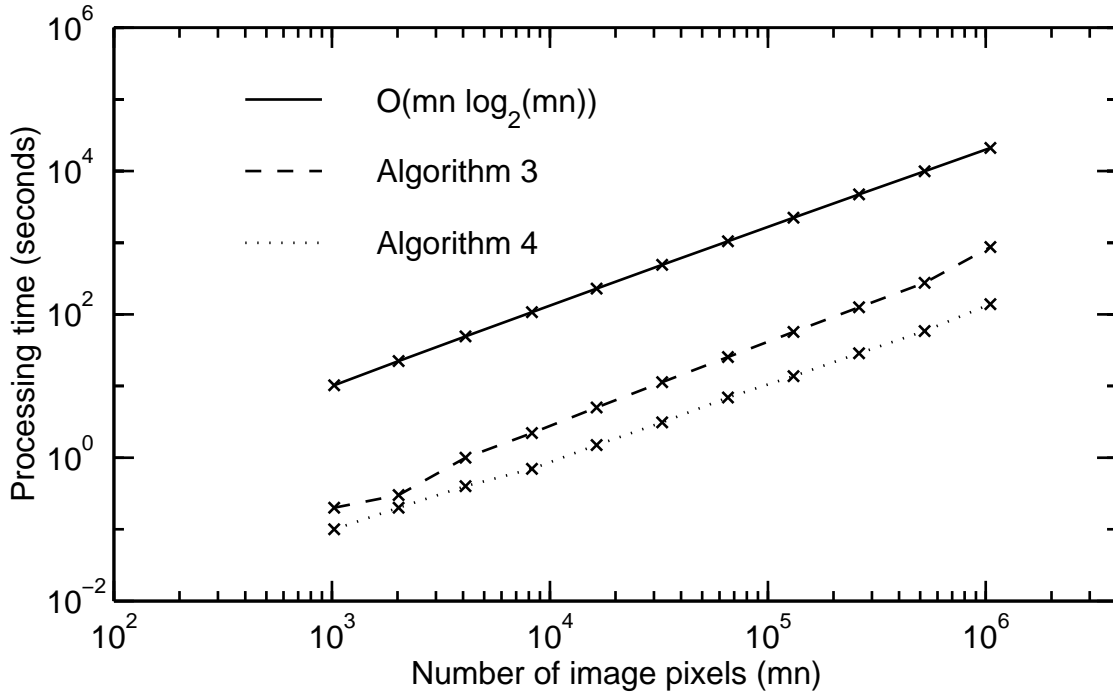
Figure 5: Typical computation times for Algorithm 3 and Algorithm 4.
