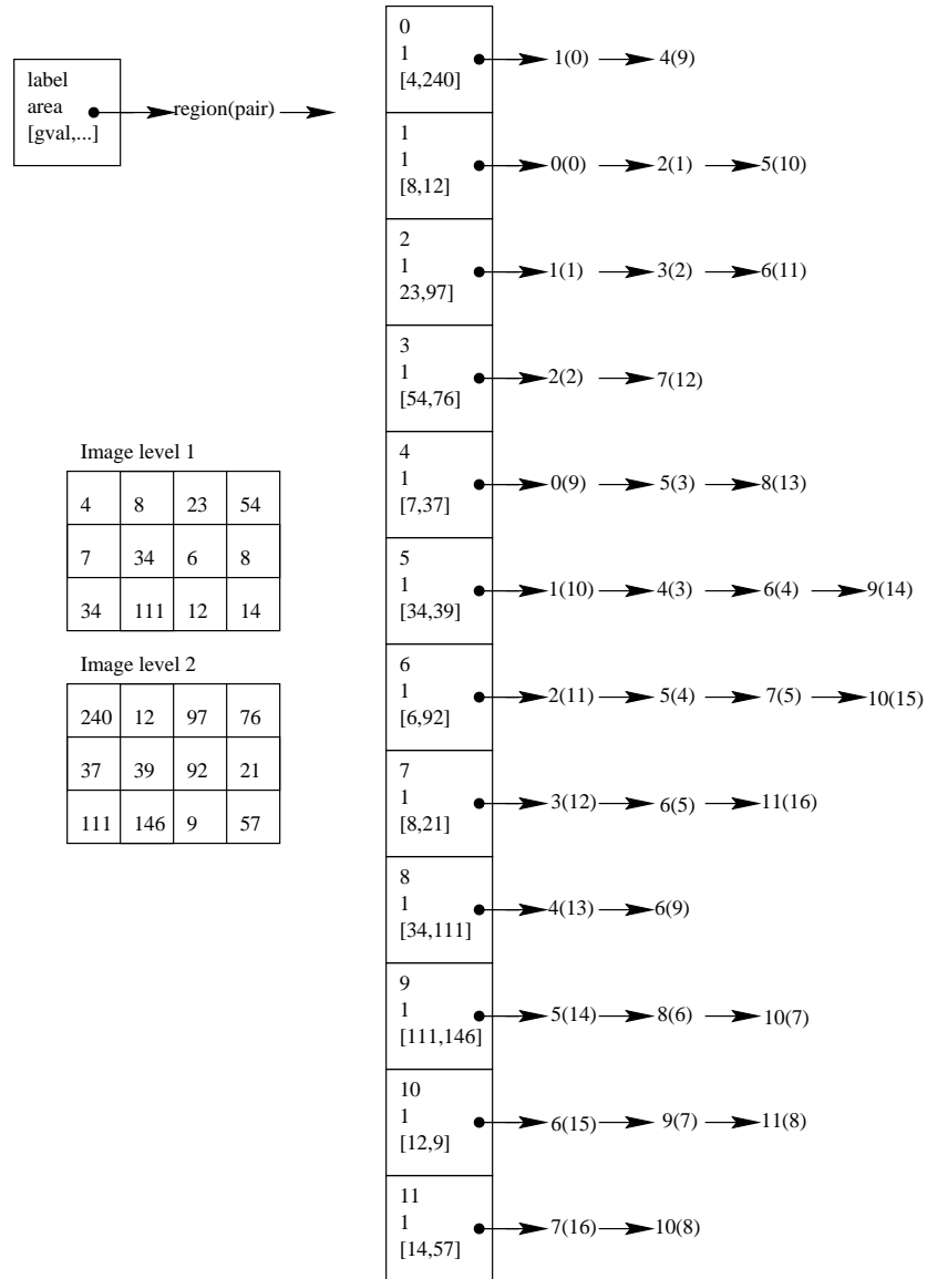
Figure 3: Structural representation of the region set for the example 3×4 2 greyscale layer image in table 1 after the trivial segmentation.
