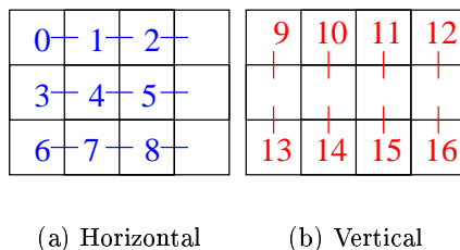
Figure 2: Labelling of the (a) horizontal, and (b) vertical pairs for the trivial segmentation of the example 3 \times 4 image.
