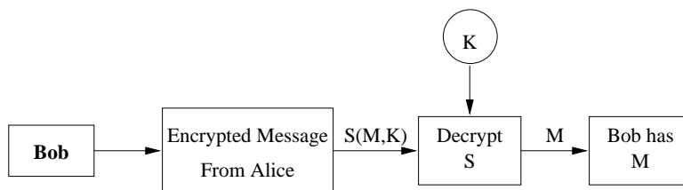
Figure 5: Bob recovers the message M .
