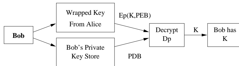
Figure 4: Bob recovers the key K.
